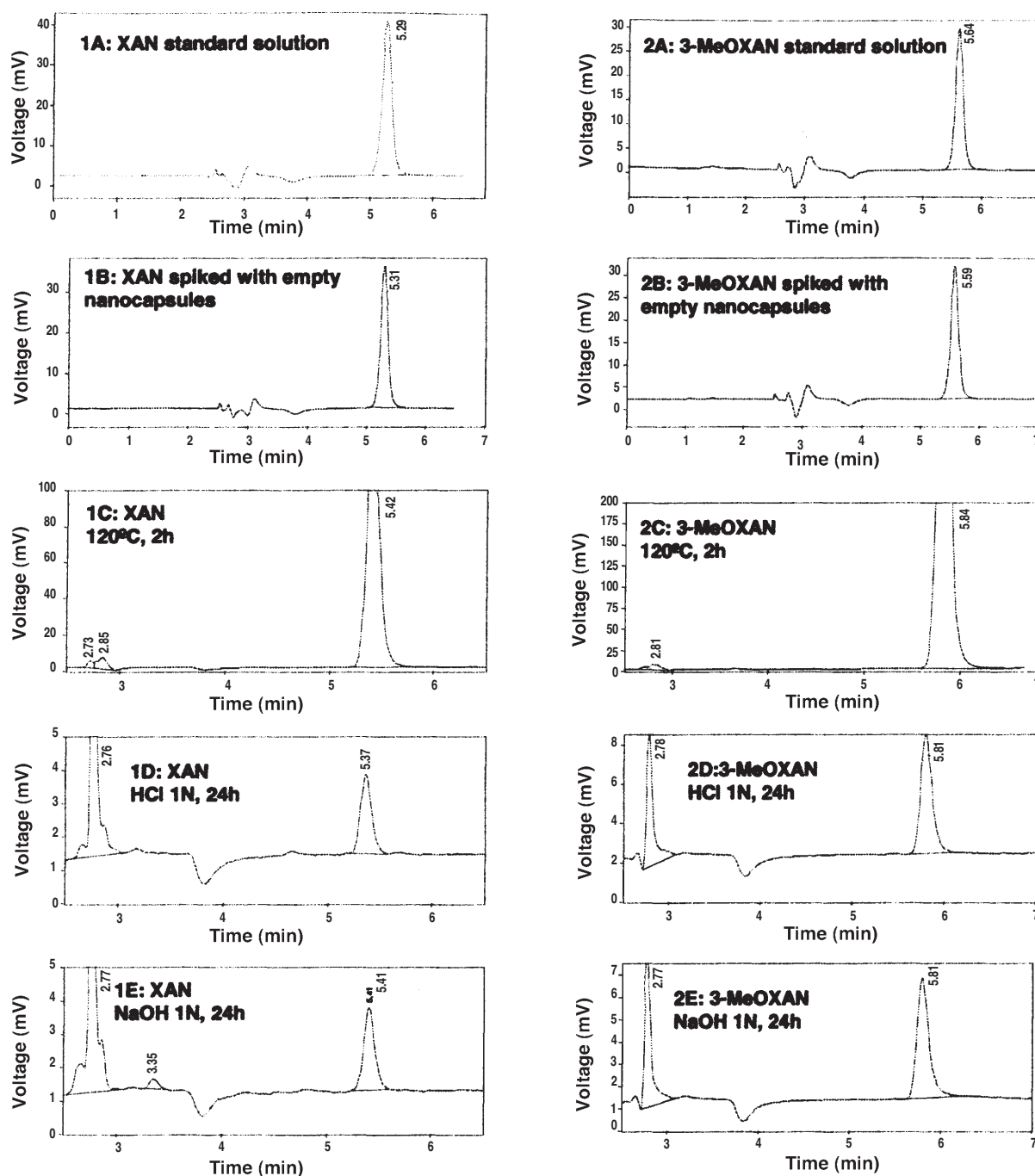
Figure 2. Representative chromatograms obtained following the injection of: (1A) XAN, 1.4 \mu\text{g}/\text{mL} ; (2A) 3-MeOXAN, 1.0 \mu\text{g}/\text{mL} ; (1B) XAN and (2B) 3-MeOXAN standard solutions spiked with empty nanocapsules; (1C) XAN and (2C) 3-MeOXAN subjected to thermal degradation, 120°C for 2 h; (1D) XAN and (2D) 3-MeOXAN subjected to acid degradation, HCl 1N for 24 h; and (1E) XAN and (2E) 3-MeOXAN subjected to basic degradation, NaOH 1N for 24 h.
